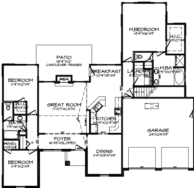
FIRST FLOOR PLAN A-C
