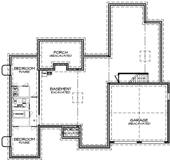
FOUNDATION PLAN A-B
